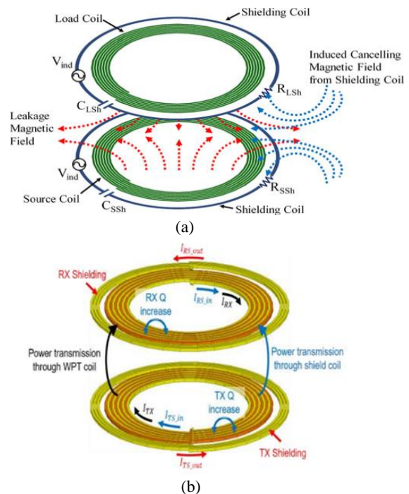
Figure 15. Shielding for WPT systems (a) active, and (b) reactive (Kim and Ahn 2021; Park et al. 2017)
