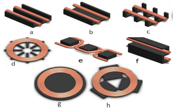
Figure 10. Some forms of Ferrite used in WPT systems: (a) E shape coil, (b) U shape coil, (c) W shape coil, (d) Split surface bars (e) I shape coil, (f) S shape coil, (g) Entire surface, (h) Split surface square (Triviño-Cabrera et al 2020).
